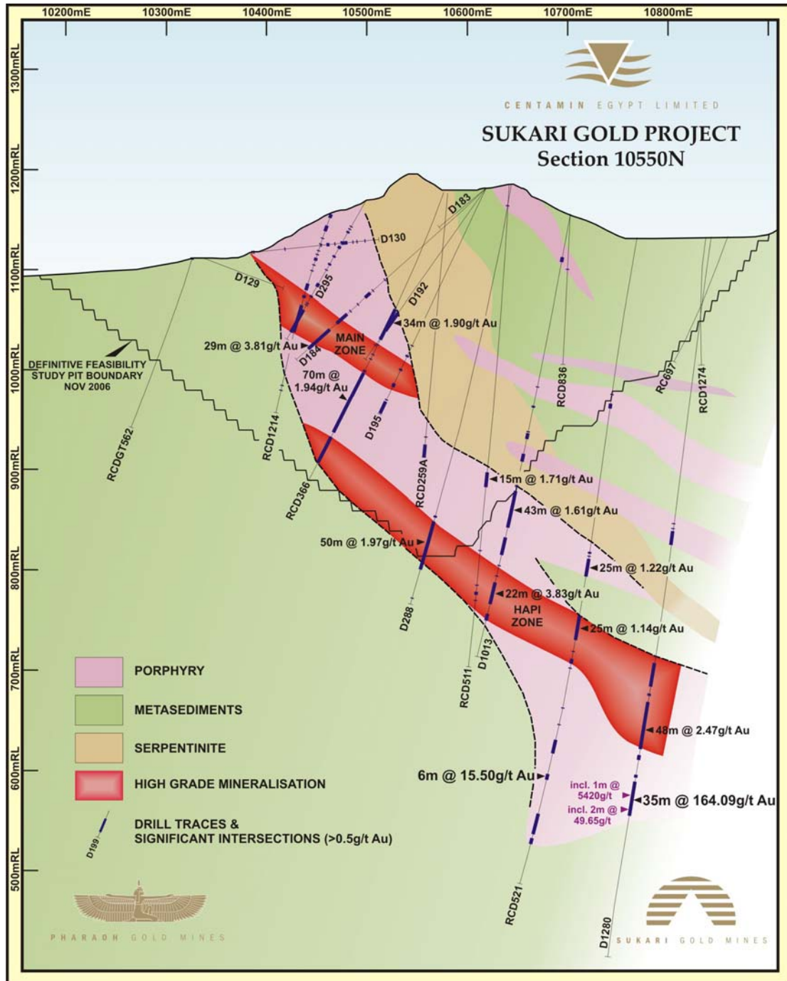
Figure 2 – Section 10550N displaying high grade zones in hole D1280
